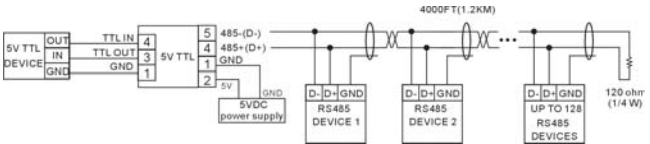
Figure 2: Master/Slave multiple drop configuration
