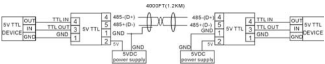
Figure 1: Extending TTL Data Distance
